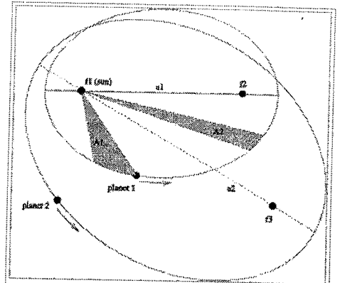
Illustration of Kepler's three laws with two planetary orbits. (1) The orbits are ellipses, with focal points f_1 and f_2 for the first planet and f_1 and f_3 for the second planet. The sun is placed in focal point f_1 . (2) The two shaded segments A_1 and A_2 have the same surface area and the time for planet 1 to cover segment A_1 is equal to the time to cover segment A_2 . (3) The total orbit times for planet 1 and planet 2 have a ratio a_1^{3/2} : a_2^{3/2} .
